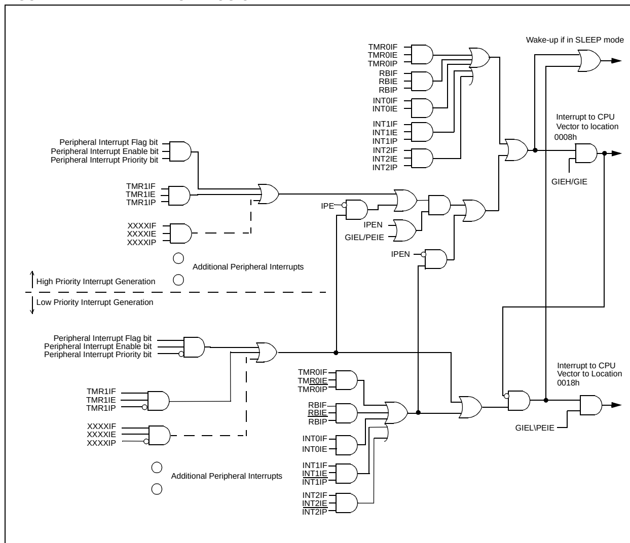
FIGURE 7-1: INTERRUPT LOGIC
